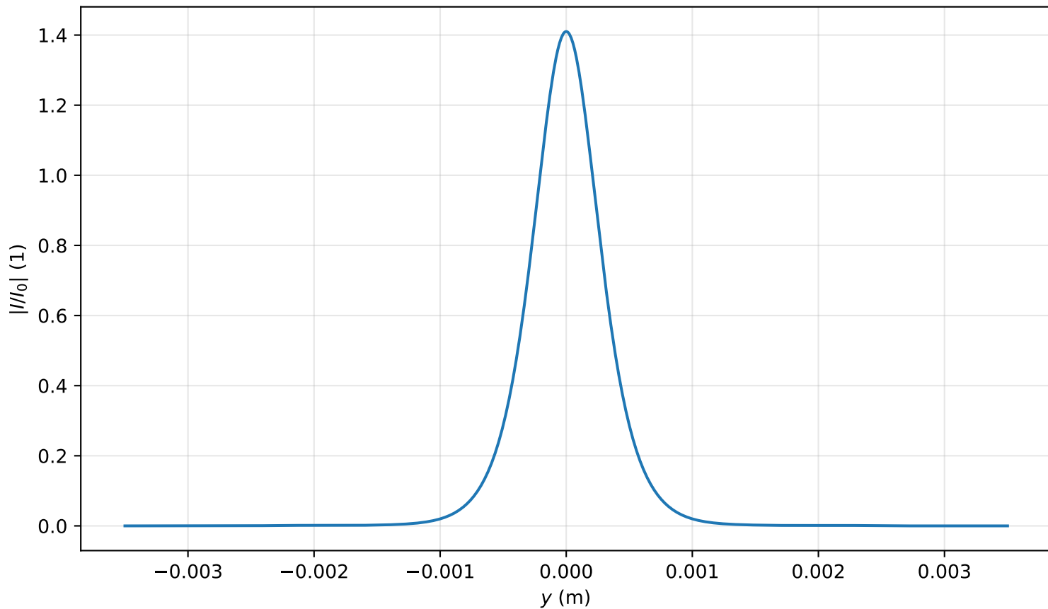
Intensity profile I(x=0, y, z=3.981)/I_0 , P_{in}=0.9P_{cr} , artificial time
